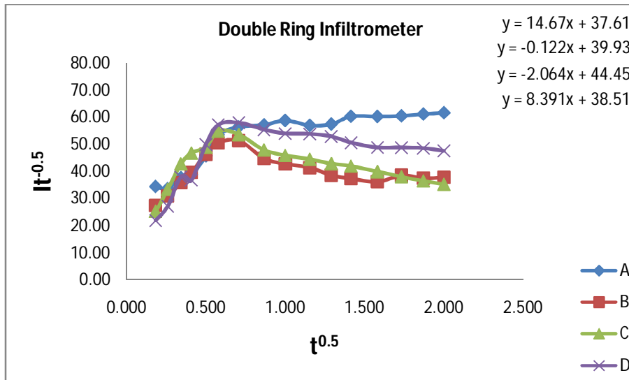
Figure 3.4: The graph of Transformed Cumulative infiltration versus transformed elapsed time to obtain the fitting parameters for Philip's equation for Double ring test.
