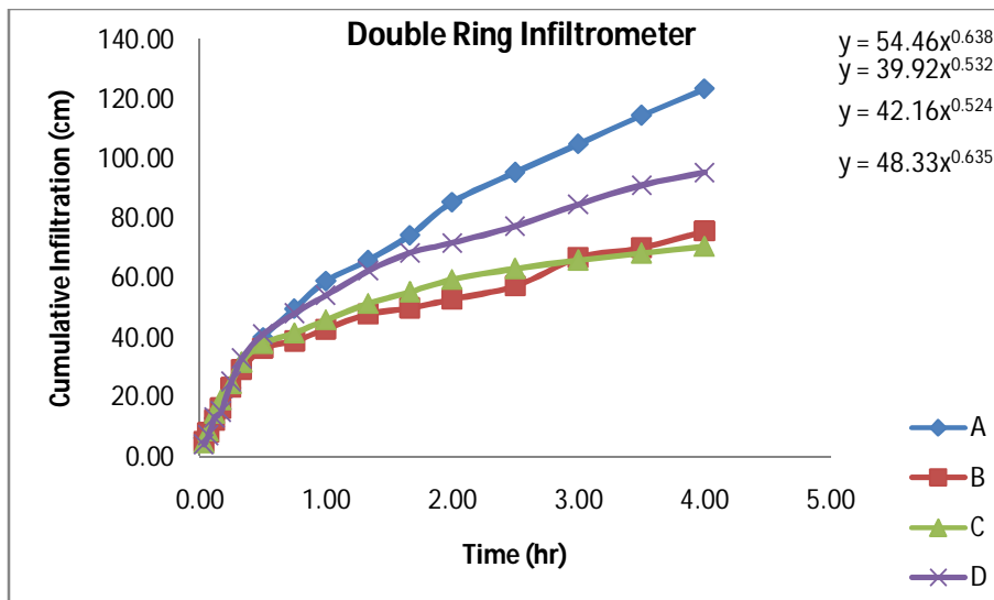
Figure 3.2: The graph of Cumulative infiltration versus elapsed time to obtain the fitting parameters for Kostiakov's equation for Double ring test.
